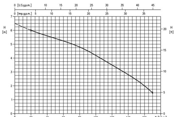
BEST ONE VOX (0.25 kW) – impeller diameter = 85 mm
